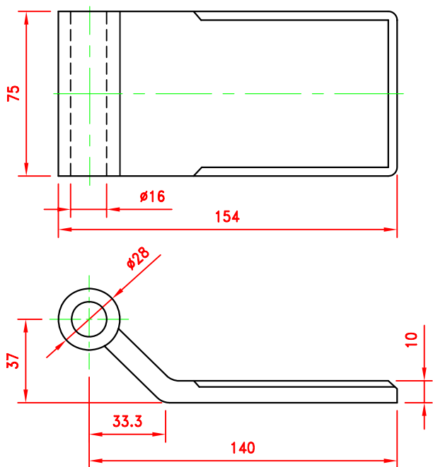
CIMC-D24-03 Welding Type
