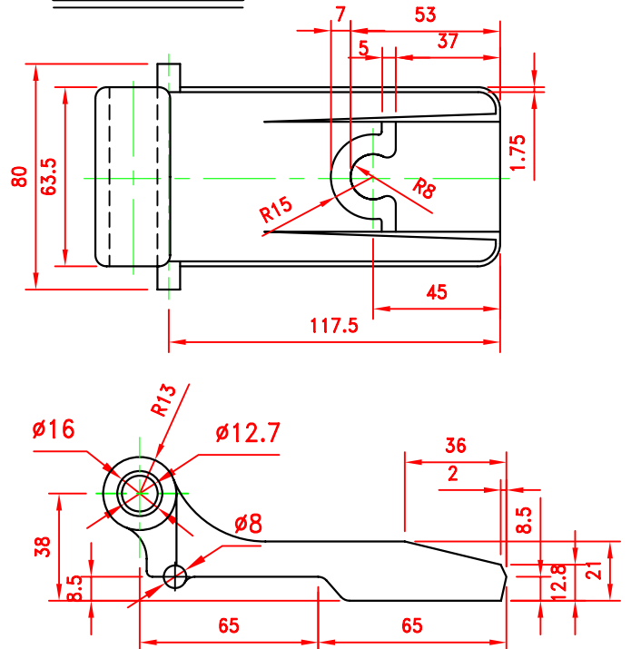
CIMC-D24-04 Maersk Type
