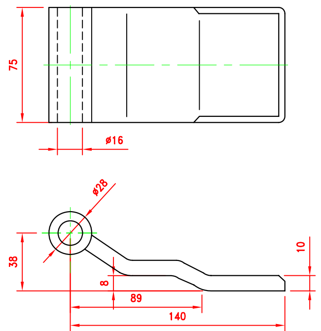
CIMC-D24-02 Welding Type
