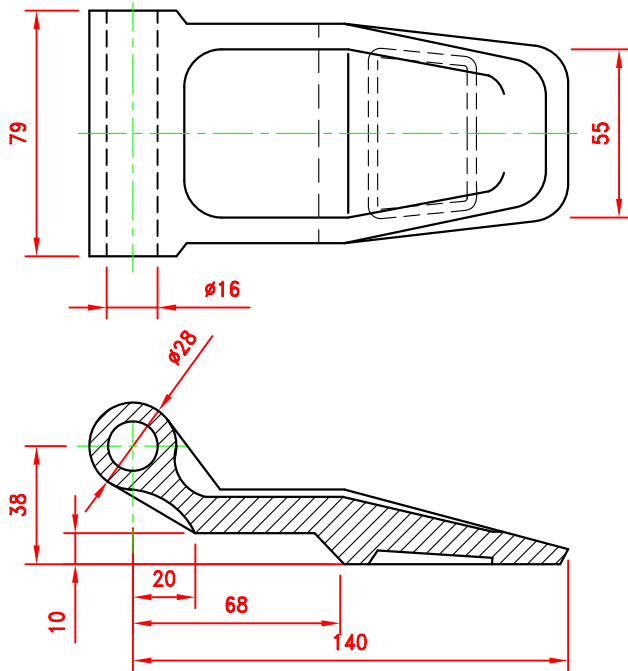
CIMC-D24-01 Froging Type
