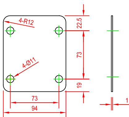
CIMC-DGE06 Large Bracket Gasket
