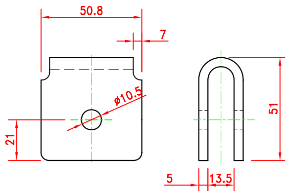
CIMC-D23-11 Handle Hub
