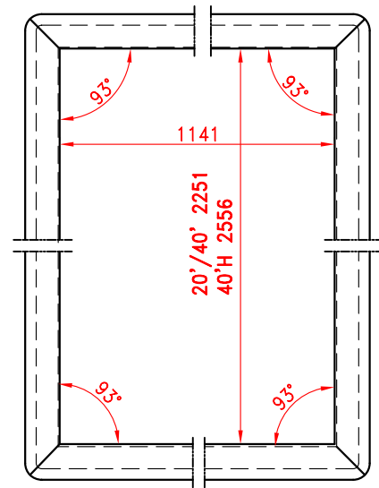
RIGHT HAND DOOR ONLY
