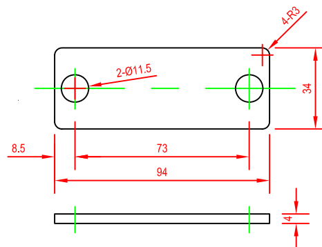
Retainer Bracket Gasket
