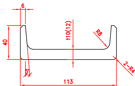
Rear Corner Post Inner 后外角柱
