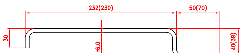
Rear Corner Post Outer 后外角柱
