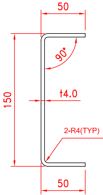
CIMC-D14-01 Door Rail
